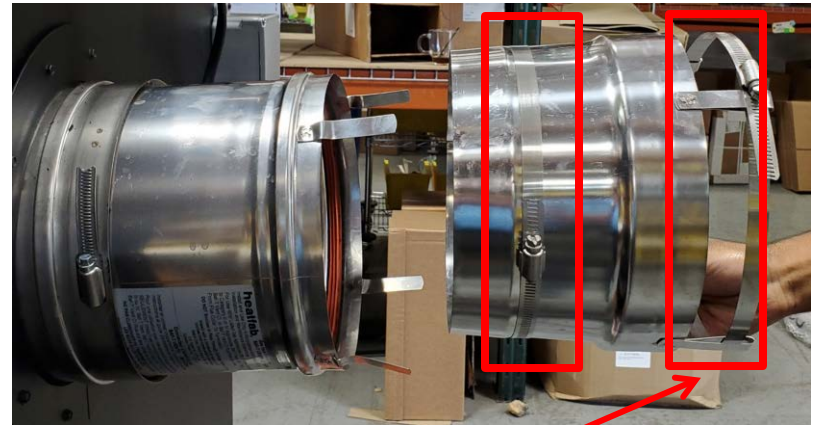
ATTACH TO CPVC VENT PIPING AND TIGHTENED CLAMP
