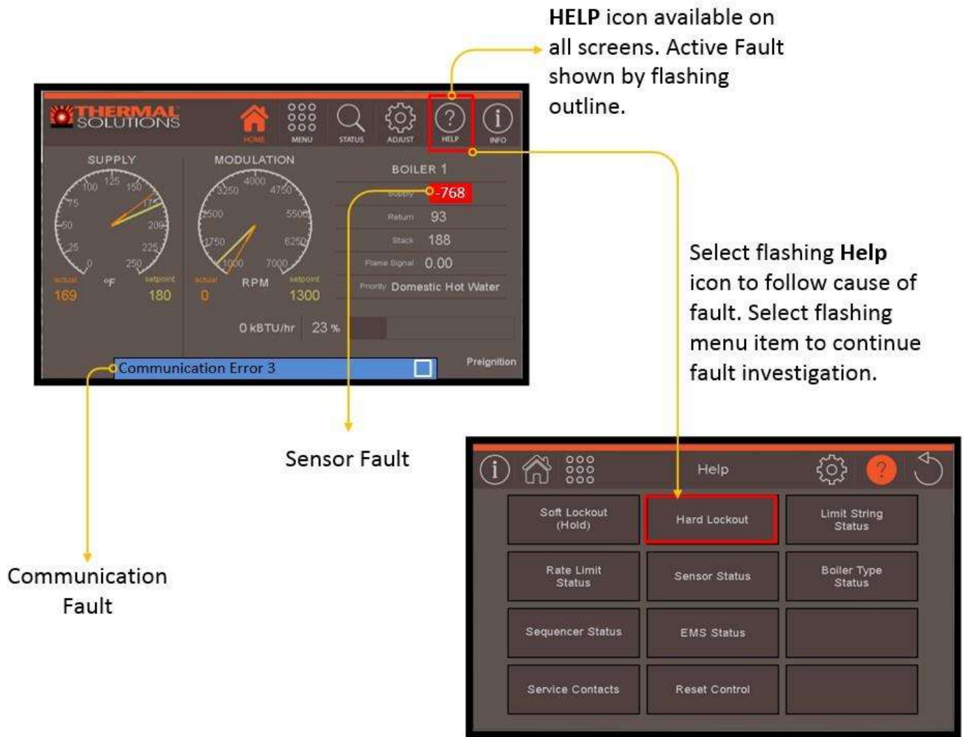
Figure 21: General Alarms
